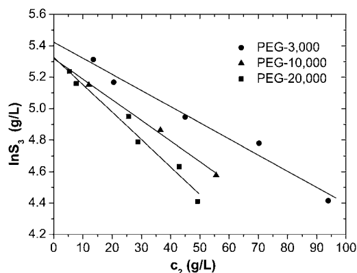
FIGURE 2 Solubility curves of lysozyme at pH = 4.0 in 0.20 M NaCl, obtained by titration with c_2 = 0.60 g/mL PEG-3000 (circles), c_2 = 0.45 g/mL PEG-10,000 (triangles), and c_2 = 0.30 g/mL PEG-20,000 (squares). Lines represent the results of least squares fit of experimental data by Eq. 5.
