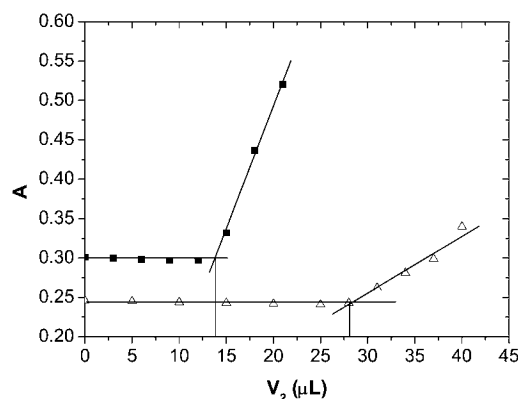
FIGURE 1 Absorbance ( \lambda = 340 nm; T = 25.0^\circ\text{C} ) during the PEG titration of lysozyme solution at pH = 4.0. Examples are shown for an initial protein solution c_3 = 190 g/L (solid symbols) and c_3 = 160 g/L (open symbols) in 0.20 M NaCl titrated with c_2 = 0.30 g/mL PEG-20,000.
